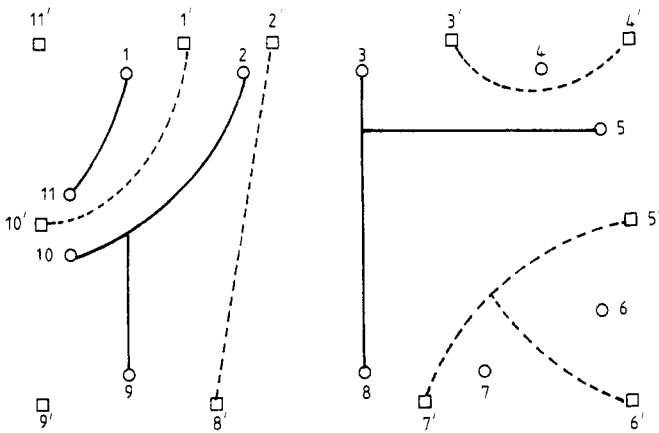
Figure 4. The partitions P = \{1, 11\}, \{2, 9, 10\}, \{3, 5, 8\}, \{4\}, \{6\}, \{7\}, Q = \{1', 10'\}, \{2', 8'\}, \{3', 4'\}, \{5', 6', 7'\}, \{9'\}, \{11'\} , and the associated forests corresponding to the partial graphs G' and D' in figure 3. Rooted vertices belonging to one block in P and Q are connected by, respectively, full and broken lines.
